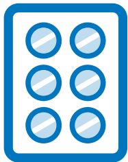
Buprenorfin
